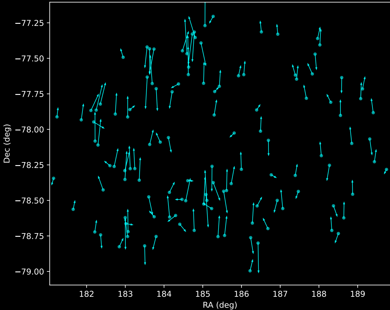
APOGEE DR17 Noise Stream Proper Motion Vectors (n=121)
