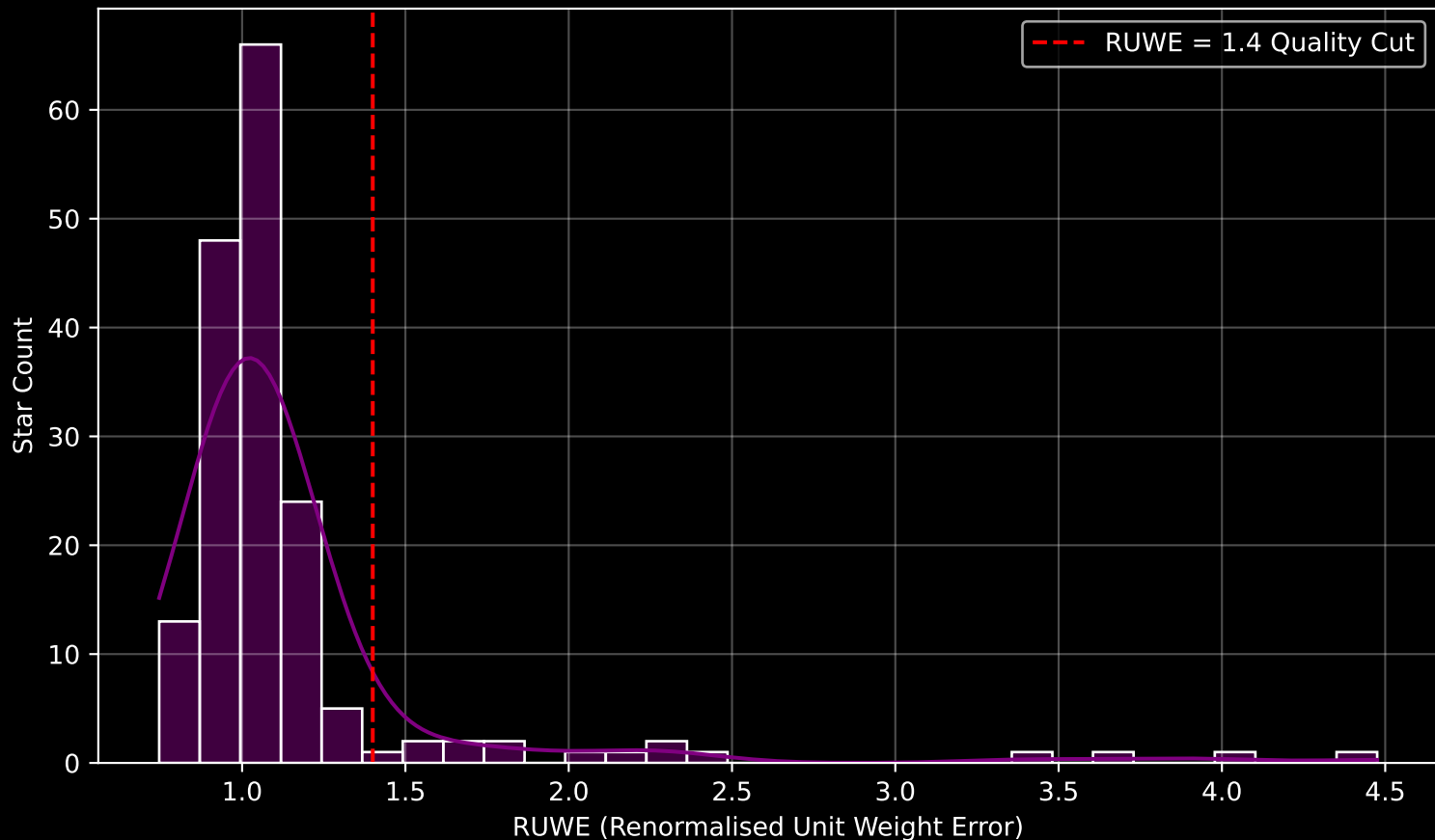
GAPOGEE DR17 Field [290-30-O_TESS] RUWE Distribution (n= 172)
