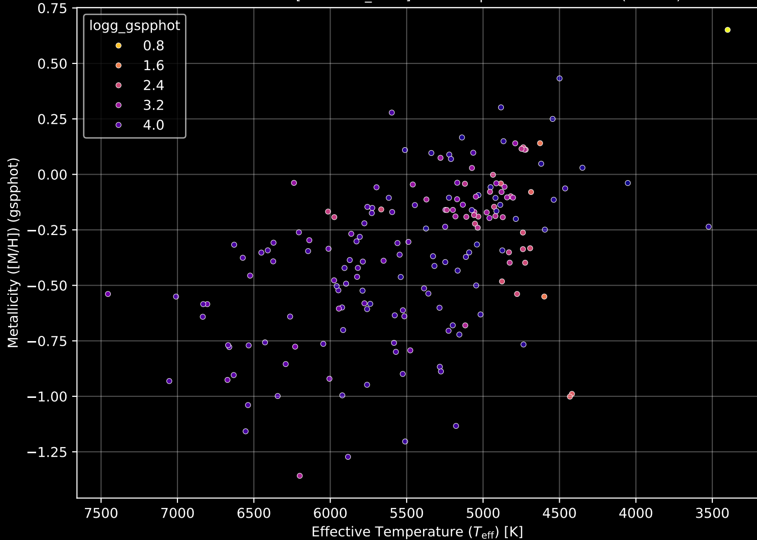
APOGEE DR17 Field: [290-30-O_TESS] Stellar Population Parameters (n= 180)
