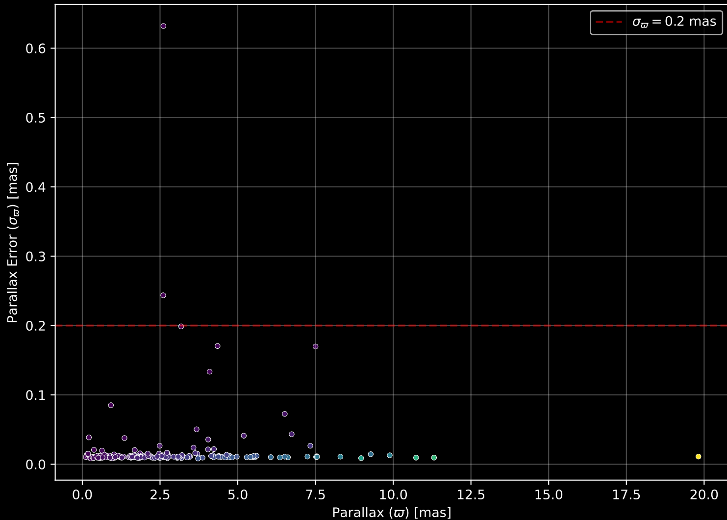
APOGEE DR17 Field: [290-30-O_TESS] Parallax Quality (n= 180)
