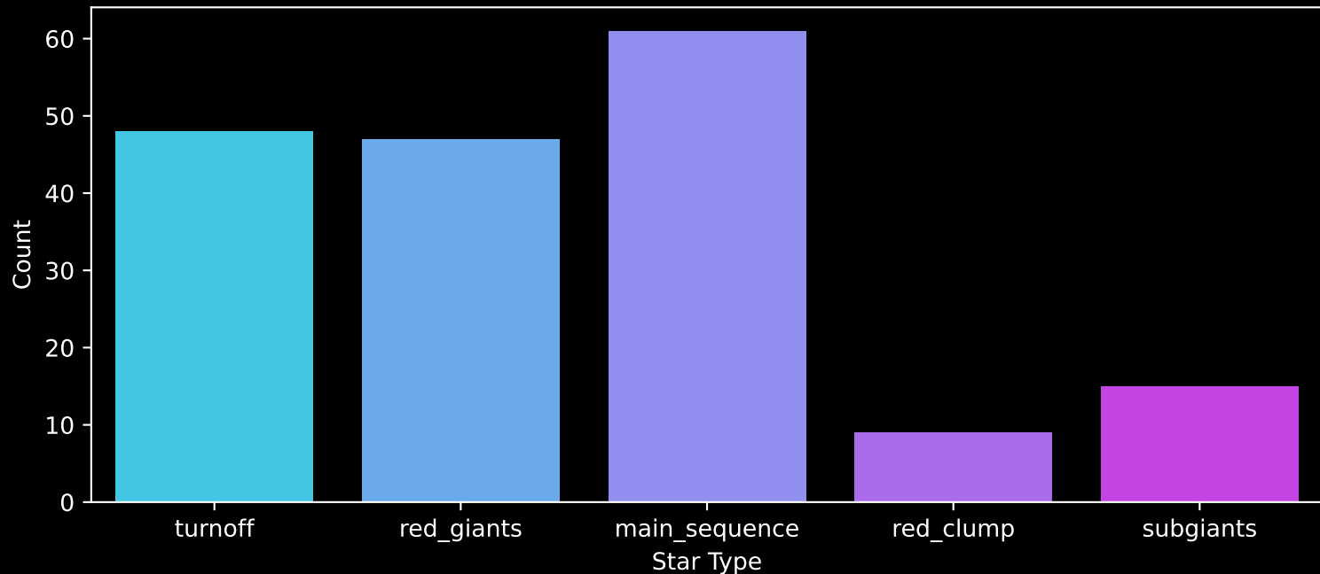
APOGEE DR17 Field: [290-30-O_TESS] Count plot of Star Type
