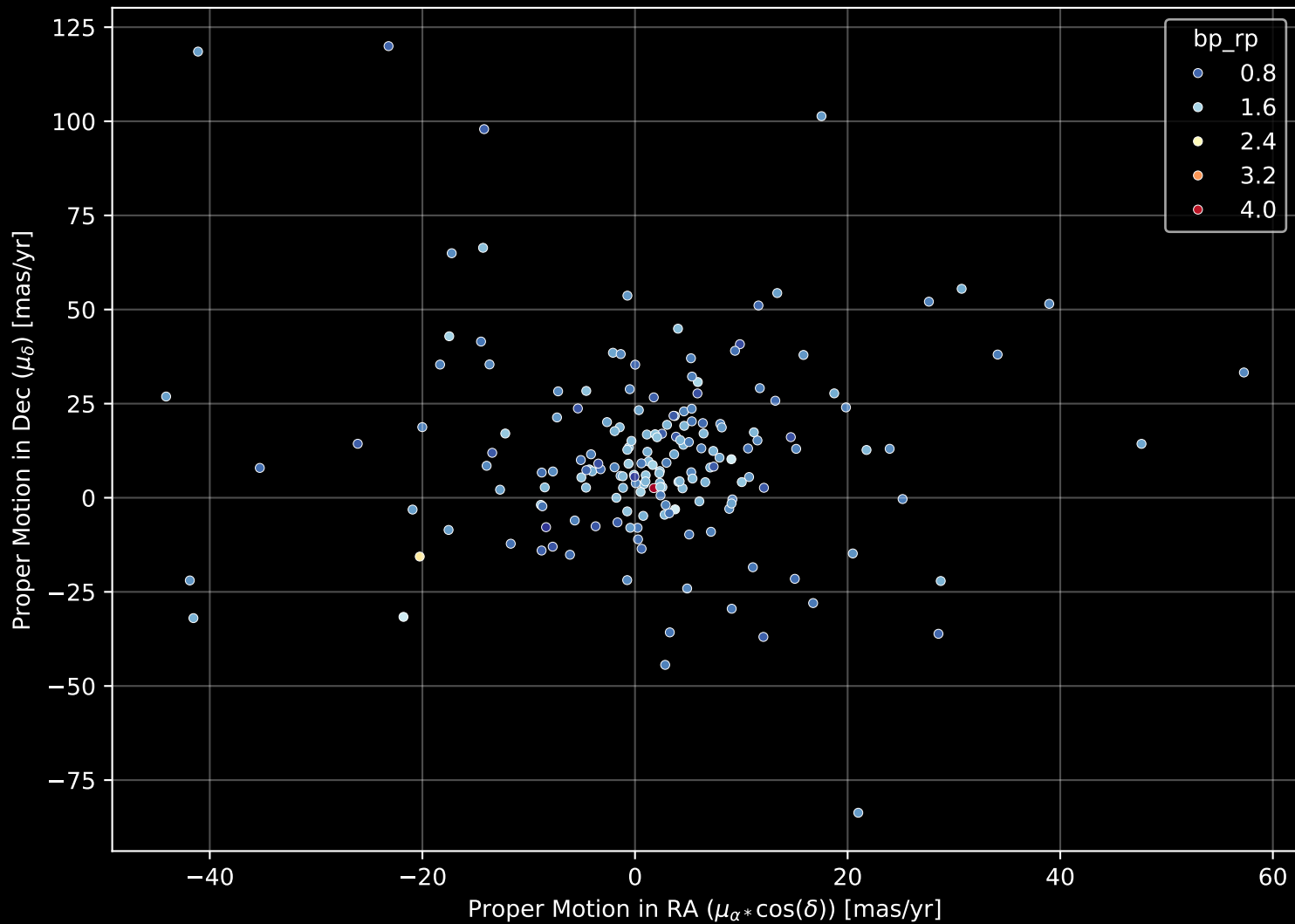
APOGEE DR17 Field: [290-30-O_TESS] Proper Motion Diagram (n= 180)
