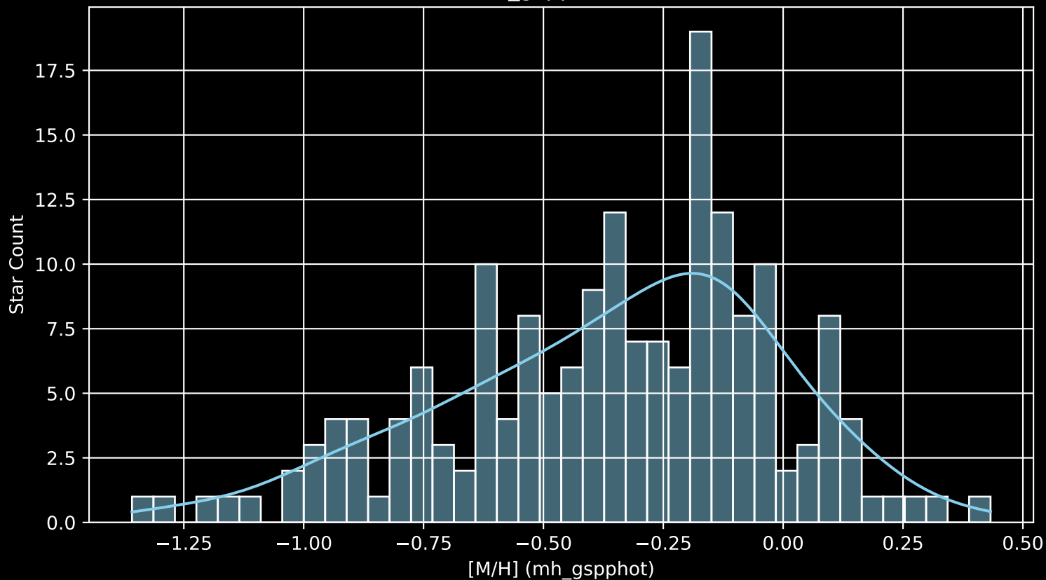
APOGEE DR17 Field: [290-30-O_TESS [M/H] (mh_gspphot) (n= 179)
