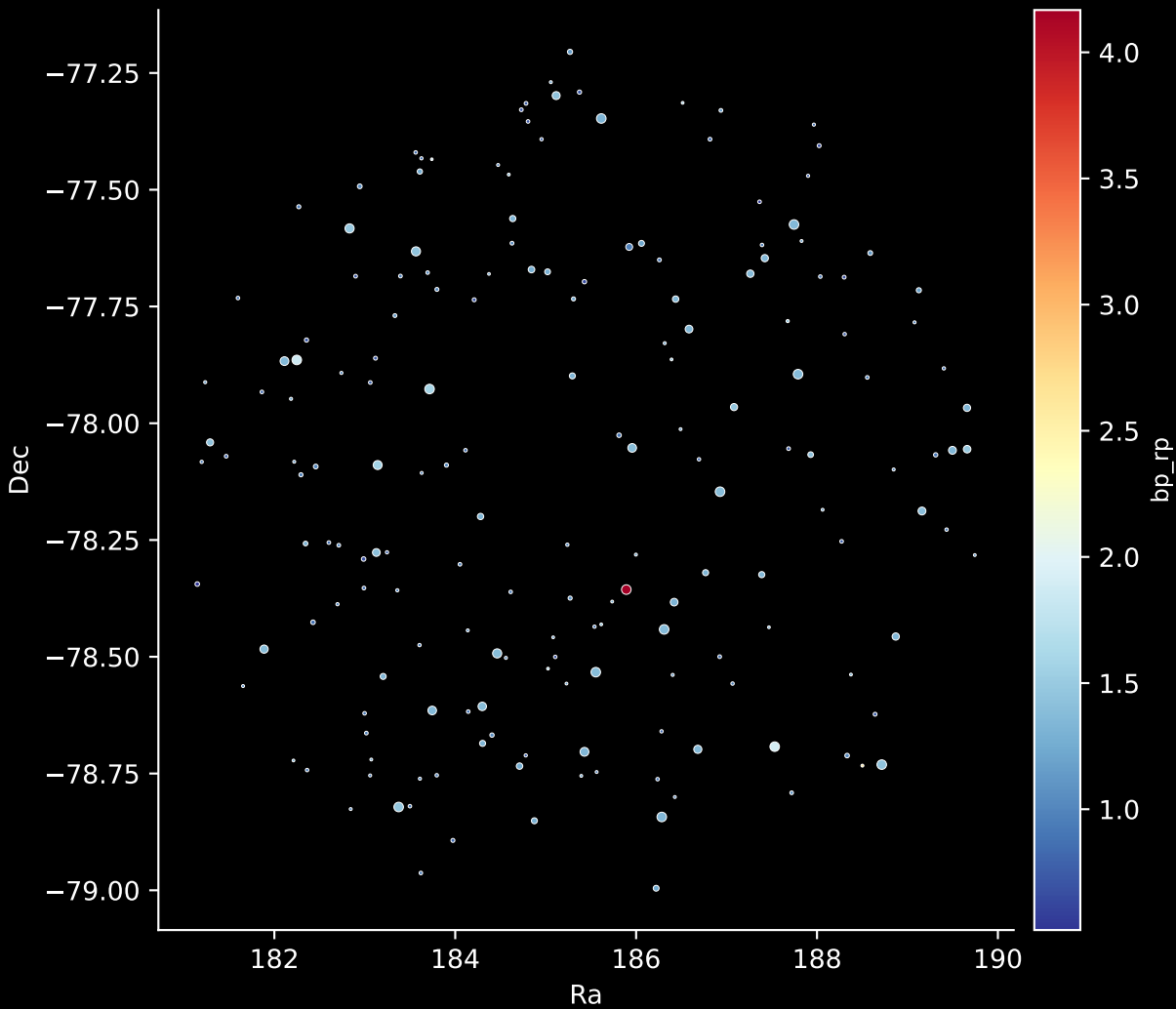
APOGEE DR17 Field: [290-30-O_TESS] Stars: 180
